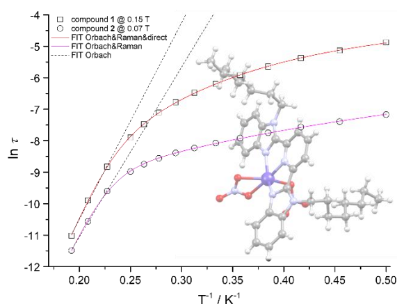
Fig. 1 Structure and \ln\tau vs 1/T dependencies of neutral field-induced Co(II)-SMMs with nitrate ligand anions
